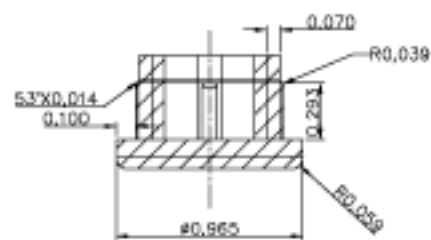
SECTION X-X
